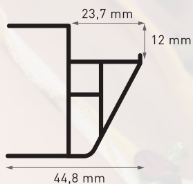
Triple 40 mm
