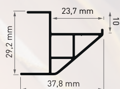
Triple
